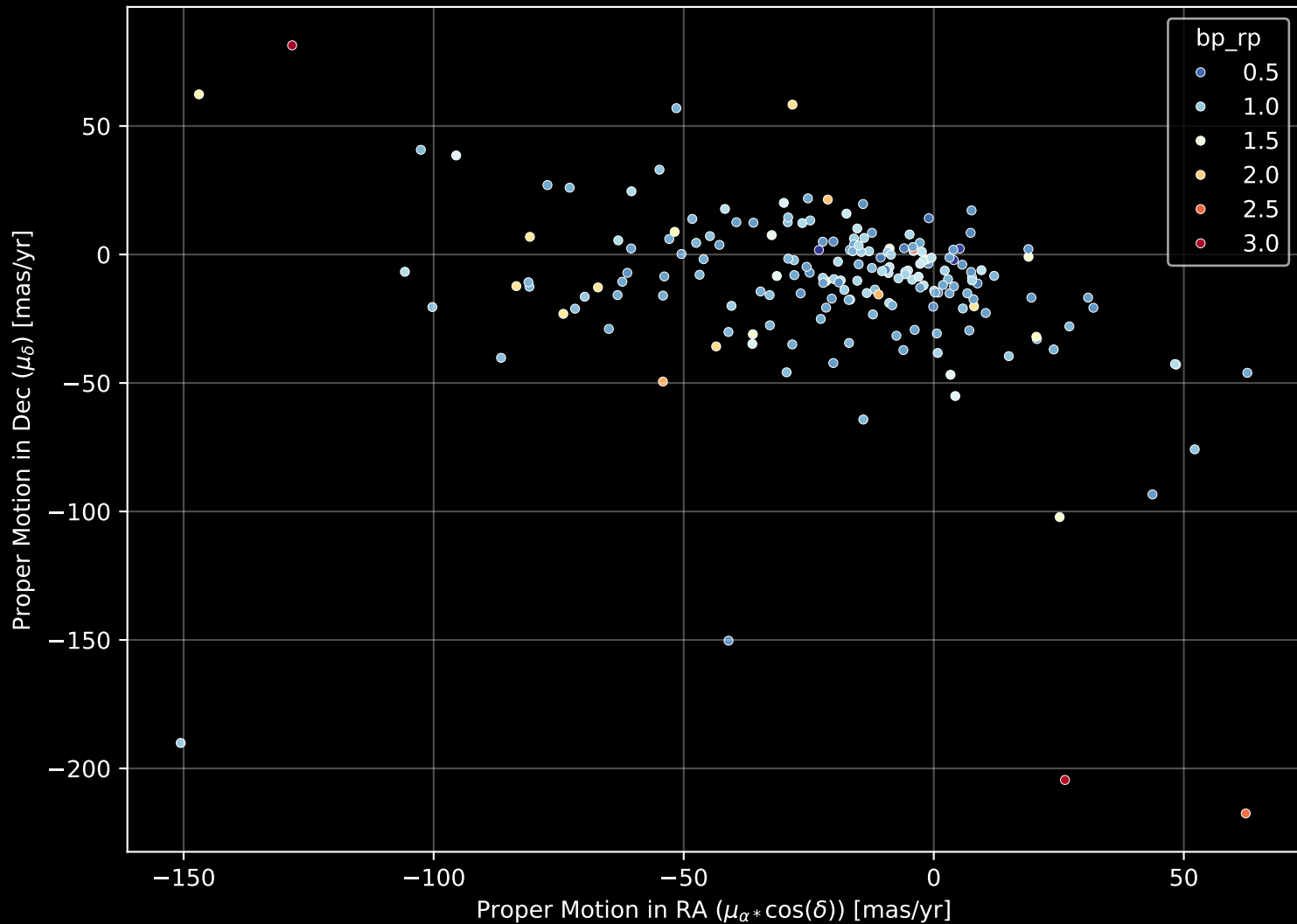
APOGEE DR17 Field: [076+88_MGA] Proper Motion Diagram (n= 191)
