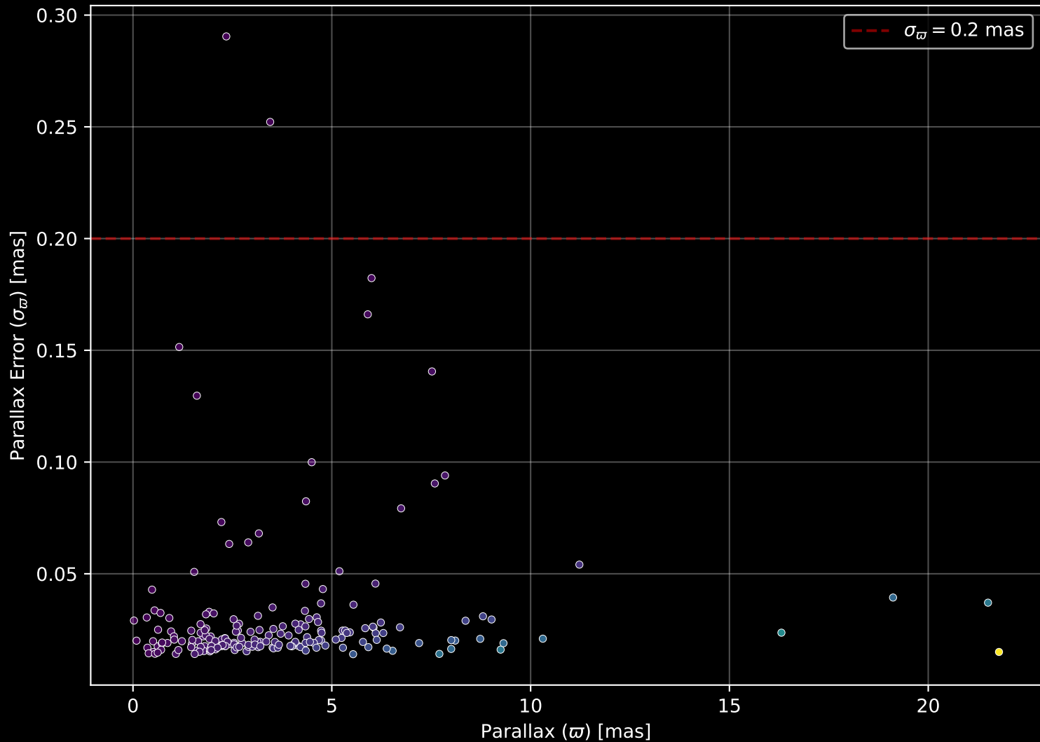
APOGEE DR17 Field: [076+88_MGA] Parallax Quality (n= 191)
