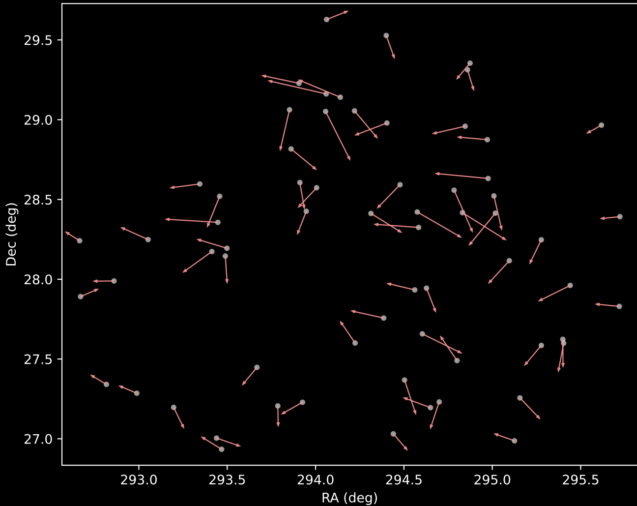
APOGEE DR17 Cluster 7 Proper Motion Vectors (n=65)
