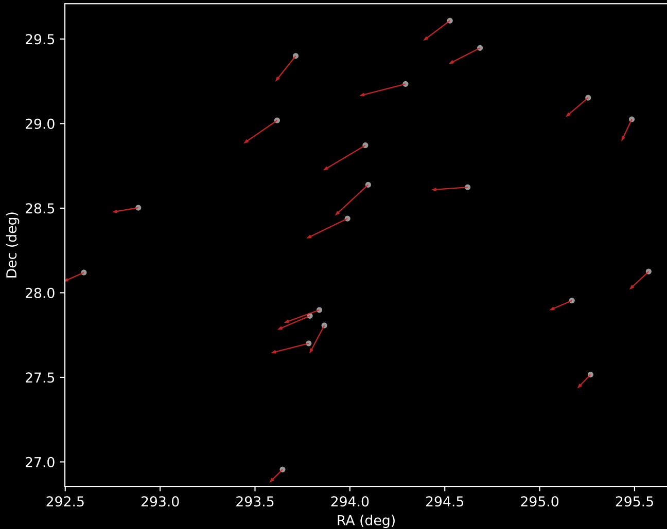
APOGEE DR17 Cluster 6 Proper Motion Vectors (n=21)
