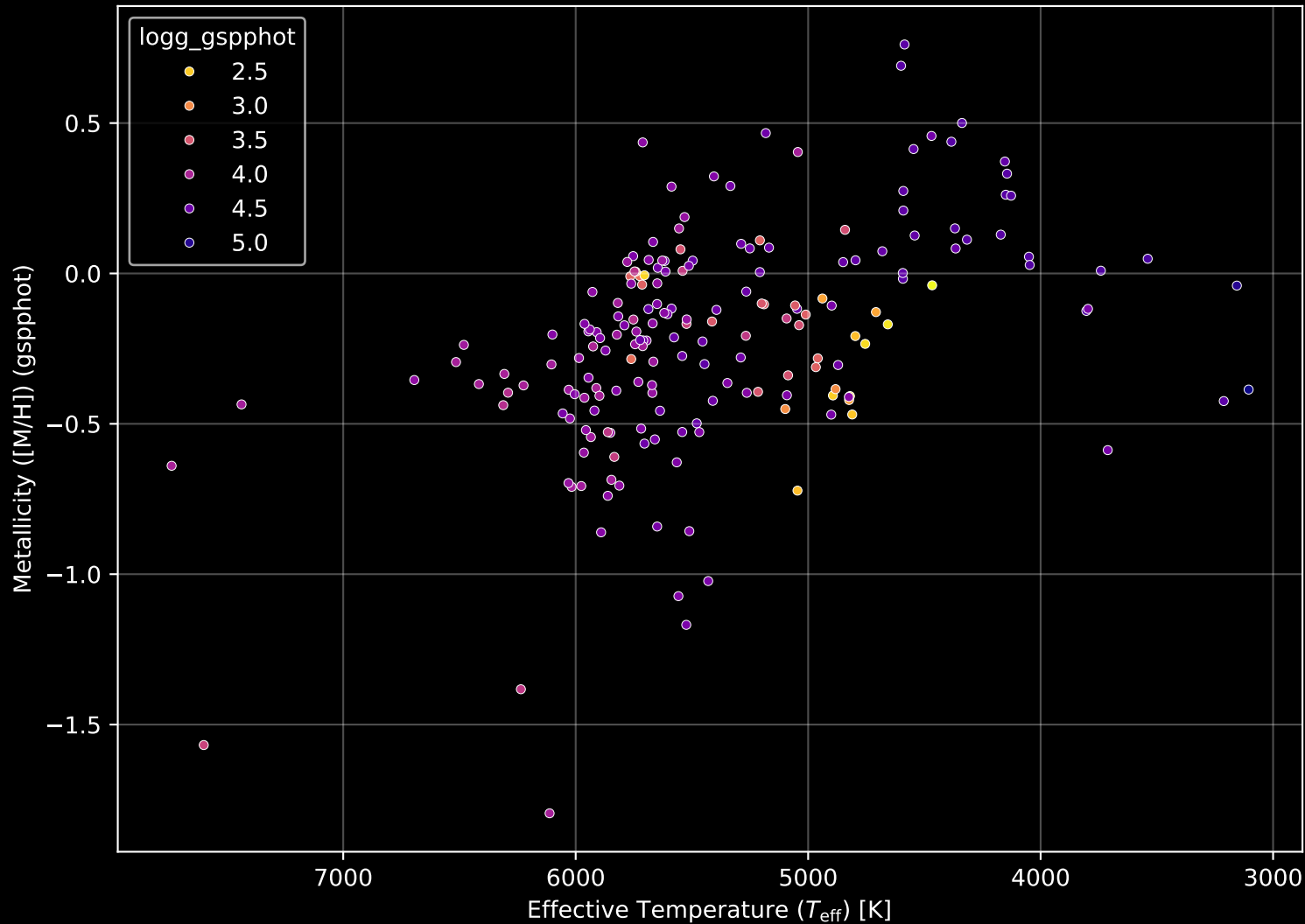
APOGEE DR17 Field: [076+88_MGA] Stellar Population Parameters (n= 191)
