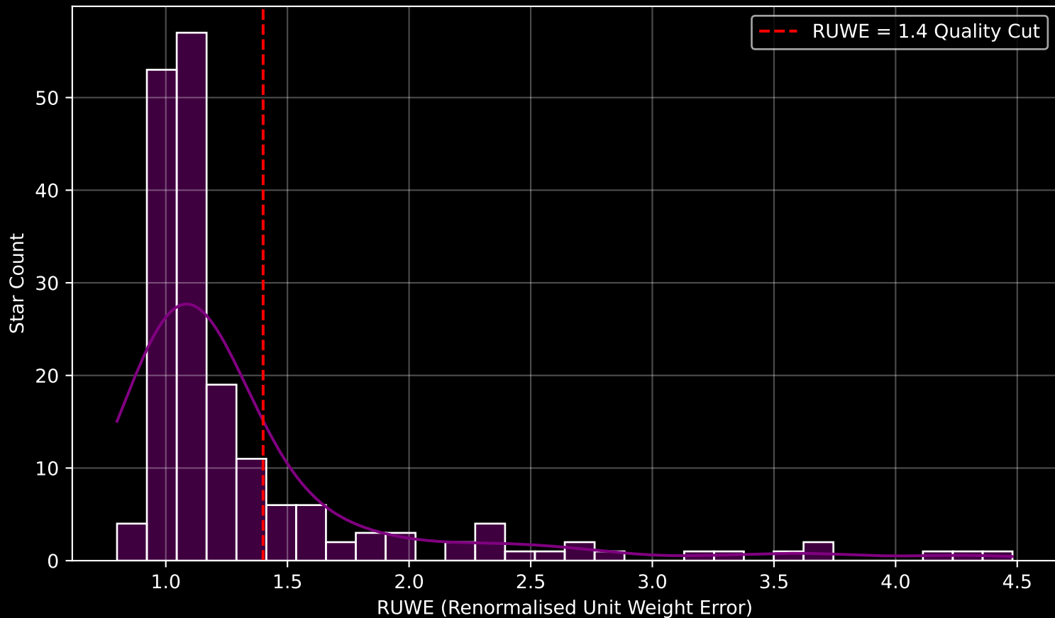
GAPOGEE DR17 Field [076+88_MGA] RUWE Distribution (n= 183)
