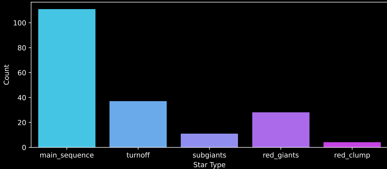
APOGEE DR17 Field: [076+88_MGA] Count plot of Star Type
