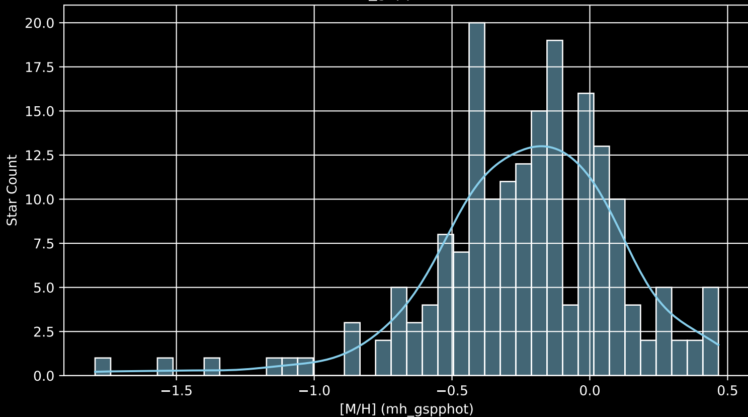
APOGEE DR17 Field: [076+88_MGA [M/H] (mh_gspphot) (n= 188)
